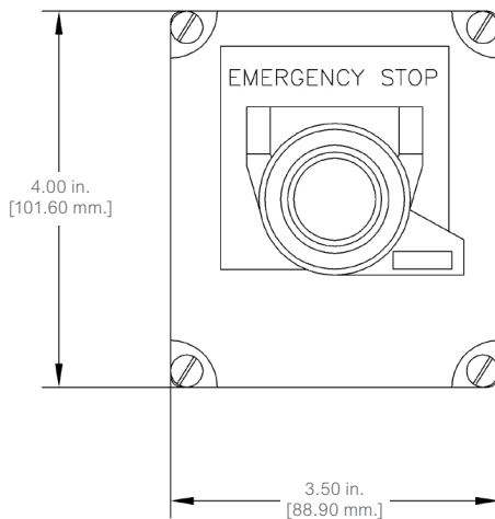
Standard Remote Fuel Shutdown Switch EM-01
