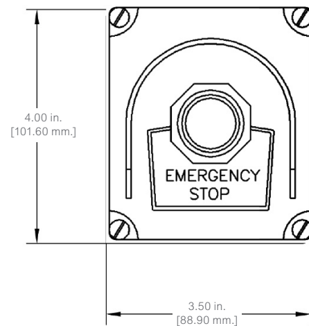
Remote Push Emergency Stop EM-01G
