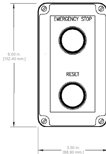
Emergency Stop Switch and Reset Switch EM-02
